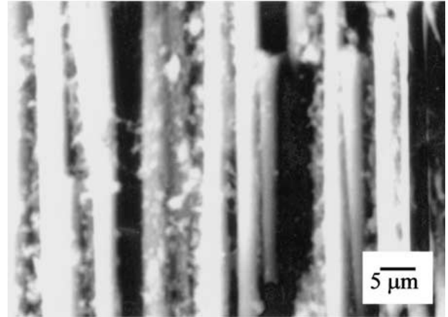
Figure 9 Scanning electron micrograph of a partially wet specimen.
