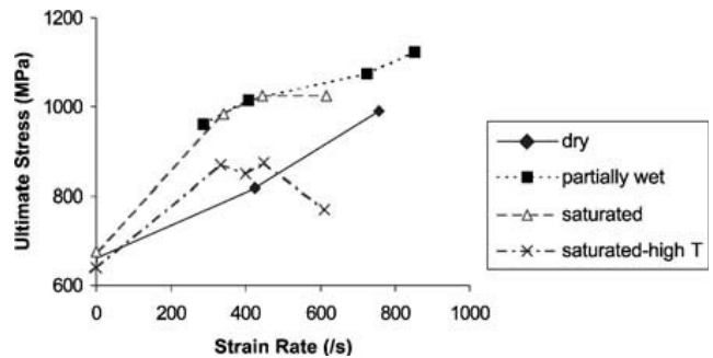
Figure 5 Ultimate stress vs. strain rate for different moisture conditions in the fiber direction.
