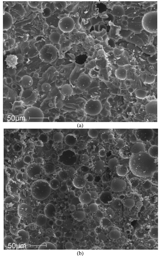
Figure 7. Fracture surface of SF460 type syntactic foams containing (a) 30% and (b) 60% microballoons.
