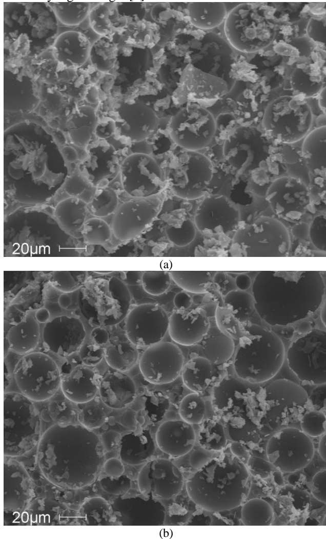
Figure 6. Fracture surface of SF220 type syntactic foams containing (a) 30% and (b) 60% microballoons.
