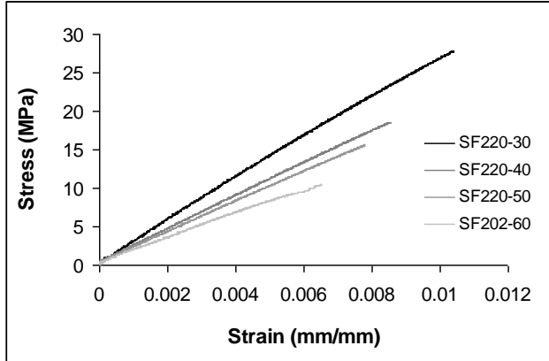
Figure 4. Representative stress-strain curves for SF220 type syntactic foams containing different volume fraction of microballoons.
