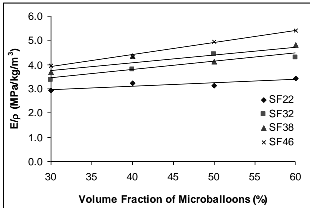
Figure 10. Comparison of specific modulus ( E/\rho ) of syntactic foams.
