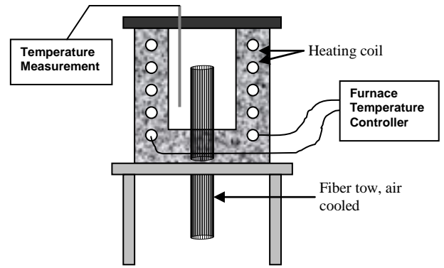
Figure 1: Experimental setup with nickel coated carbon fiber as reinforcement. The fiber bundle is extended out of the mold and air cooled during solidification.
