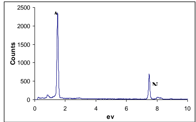
Figure 10. EDS spectrum of the white spot in the matrix showing the presence of Al and Ni, thereby indicating the presence of Ni-based compounds.
