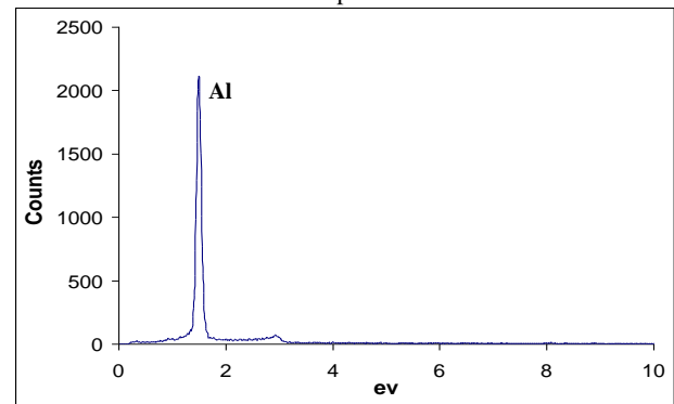
Figure 11: EDS spectrum of the matrix in the reinforced section of the squeeze infiltrated sample showing the presence of Aluminum only.
