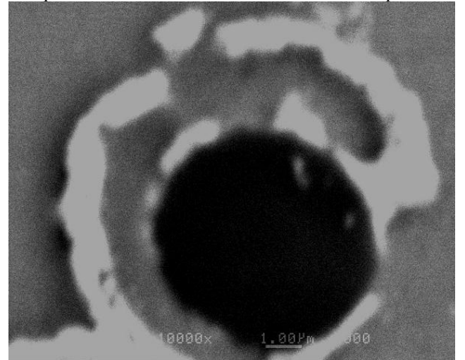
Figure 5: High Magnification SEM micrograph of squeeze cast sample showing the exfoliation and fracture of Ni coating from the carbon fiber.
