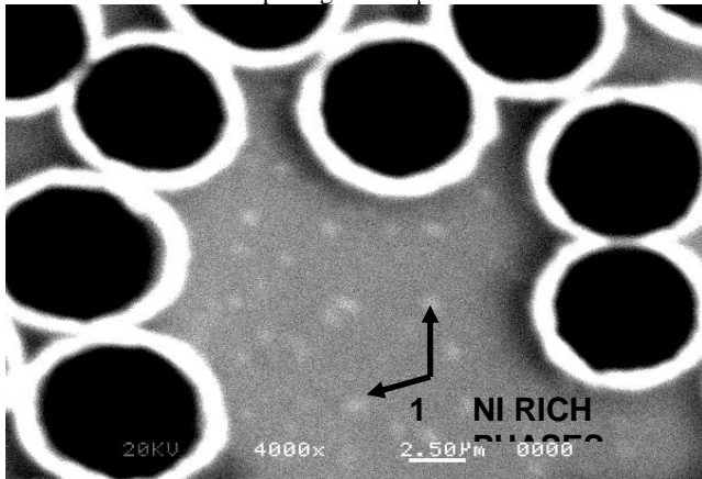
Figure 9. SEM micrograph of squeeze cast sample highlights nickel rich phases.
