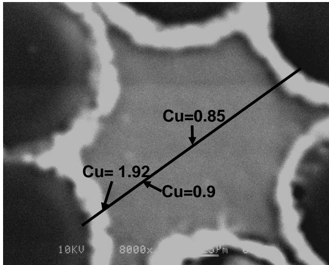
Figure 7. SEM micrograph of a squeeze cast sample. The Cu count (%) is shown at 3 different locations in the micrograph for an interfiber spacing of 13.1 \mu\text{m} .
