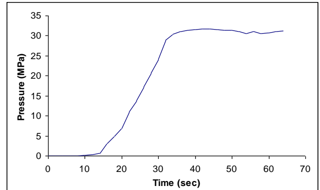
Figure 2: Recorded pressure-time cycle during squeeze infiltration of Ni coated Carbon fiber with molten Al2014 alloy.
