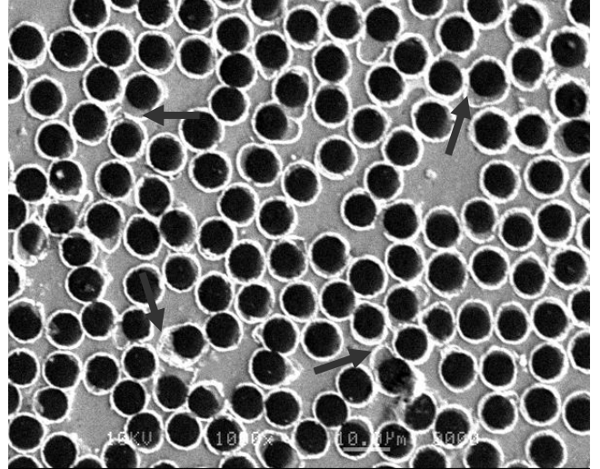
Figure 4. A micrograph showing the retention of Ni coating in squeeze infiltrated Ni coated carbon fiber-2014 composite.
