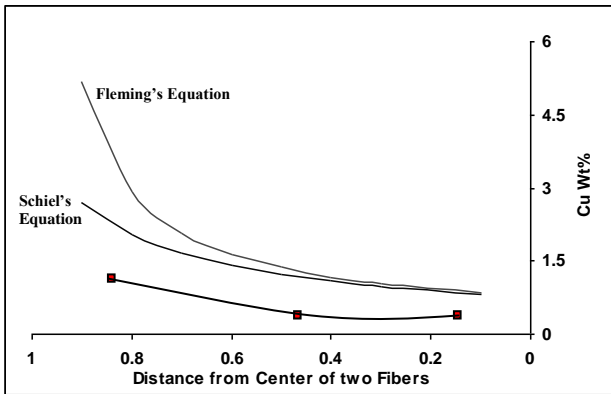
Figure 8. Comparison of copper content measured using EDS with predictions from Scheil and Fleming equations. The interfiber spacing is 18.8 \mu\text{m} .
