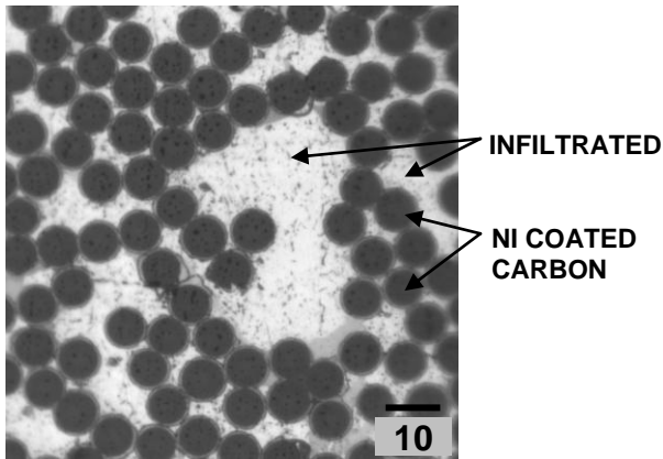
Figure 6: Micrograph of an infiltrated sample showing complete infiltration of the fiber preform.
